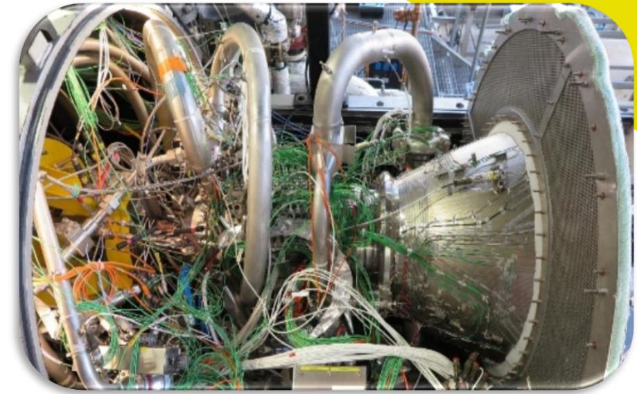
Laser Ignition technology from Austria, an ARIANE 6 engine demonstrator (Image credit: Ariane Group Holding)
